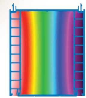
Thermography showing the heat distribution across a 100 mm StyroClick extension profile.
