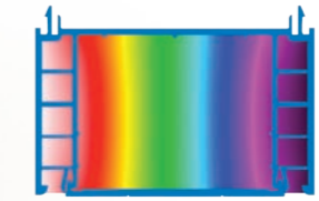
Thermographic cross-section of a 50 mm StyroClick extension profile.
